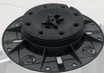
Art.nr PSTK 5474/4 Prosupport Tube System 49-74 mm, 4 mm fug - Kit à 20 stk
